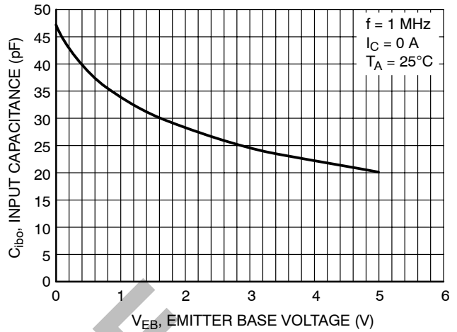
Figure 8. Input Capacitance
