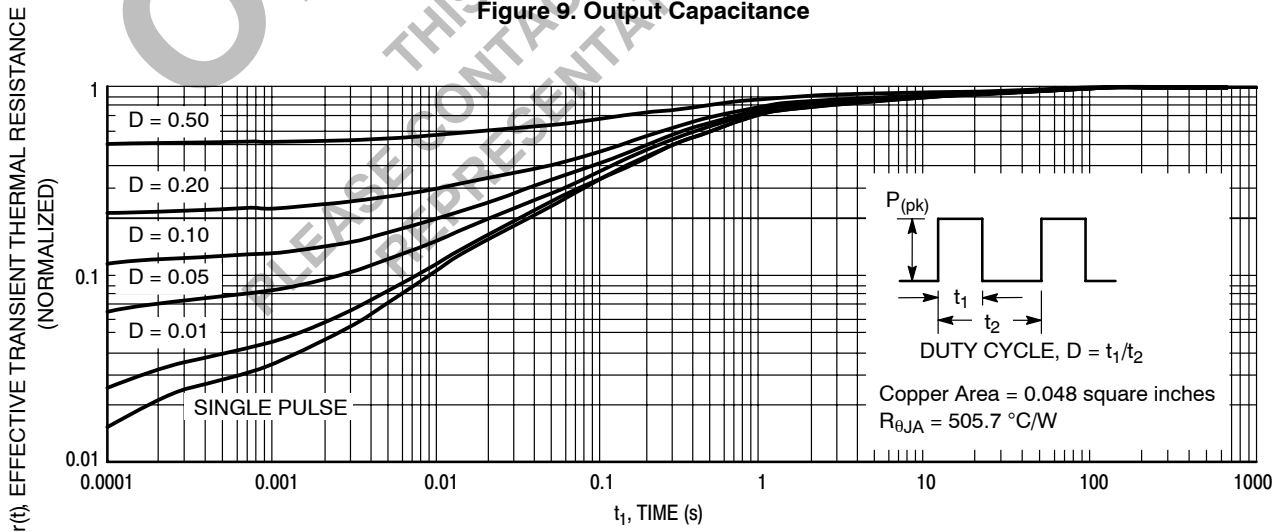
Figure 10. Normalized Thermal Response
